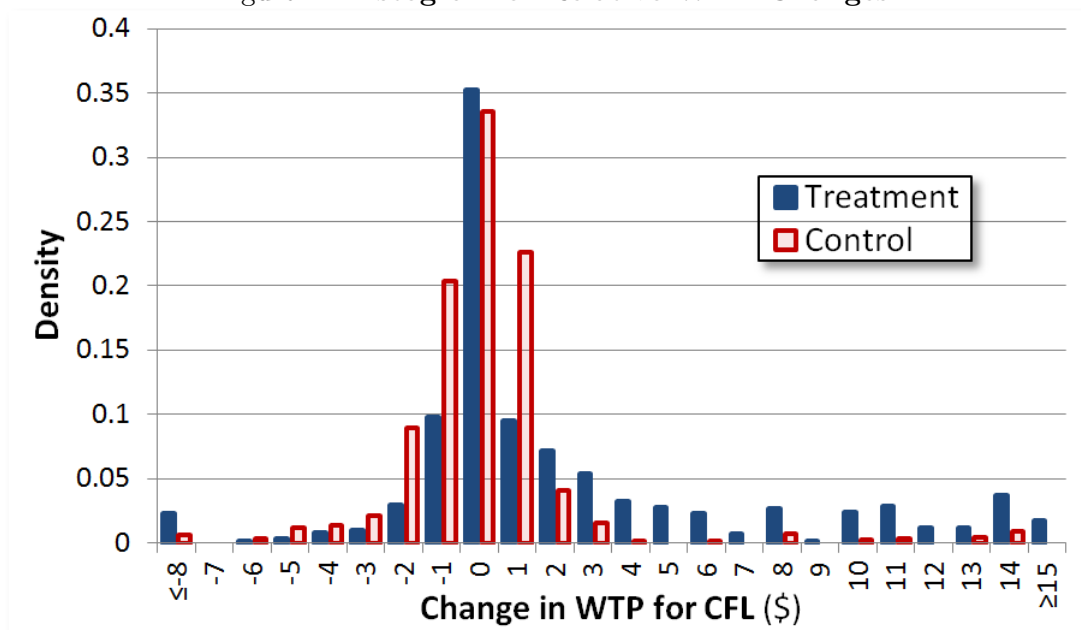
Figure 2: Histogram of Relative WTP Changes
